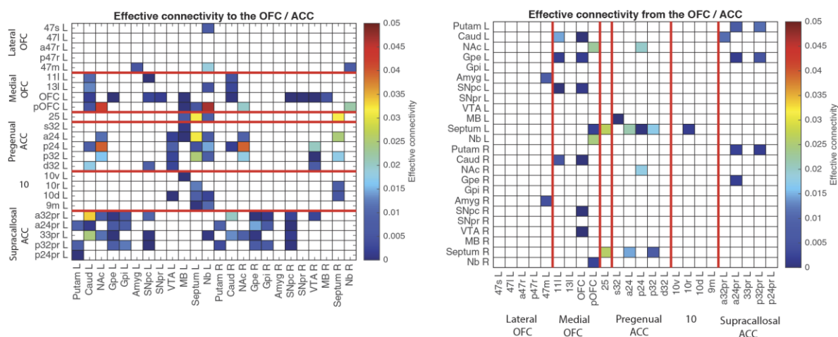
Fig. S5. Effective connectivity To (left) the OFC/ACC regions from subcortical regions; and From (right) The OFC/ACC regions to subcortical regions defined in the HCPex atlas (Huang et al. 2021a). The effective connectivity is read from column to row. Abbreviations: Putam -putamen; Caud – caudate nucleus; NAc – nucleus accumbens; GPe – globus pallidus pars externa; GPi – globus pallidus pars interna; Amyg – amygdala; SNpc – substantia nigra pars compacta; SNpr – substantia nigra pars reticulata; VTA – ventral tegmental area; MB – mammillary bodies; Nb – forebrain basal magnocellular nucleus of Meynert; L – left; R – right. Other abbreviations are shown in Table S1.
