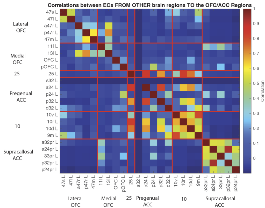
Fig. S4. Correlations between the effective connectivities from cortical areas to different regions in the orbitofrontal cortex and anterior cingulate cortex. Abbreviations: see Table S1; 25 – subgenual cingulate cortex.
