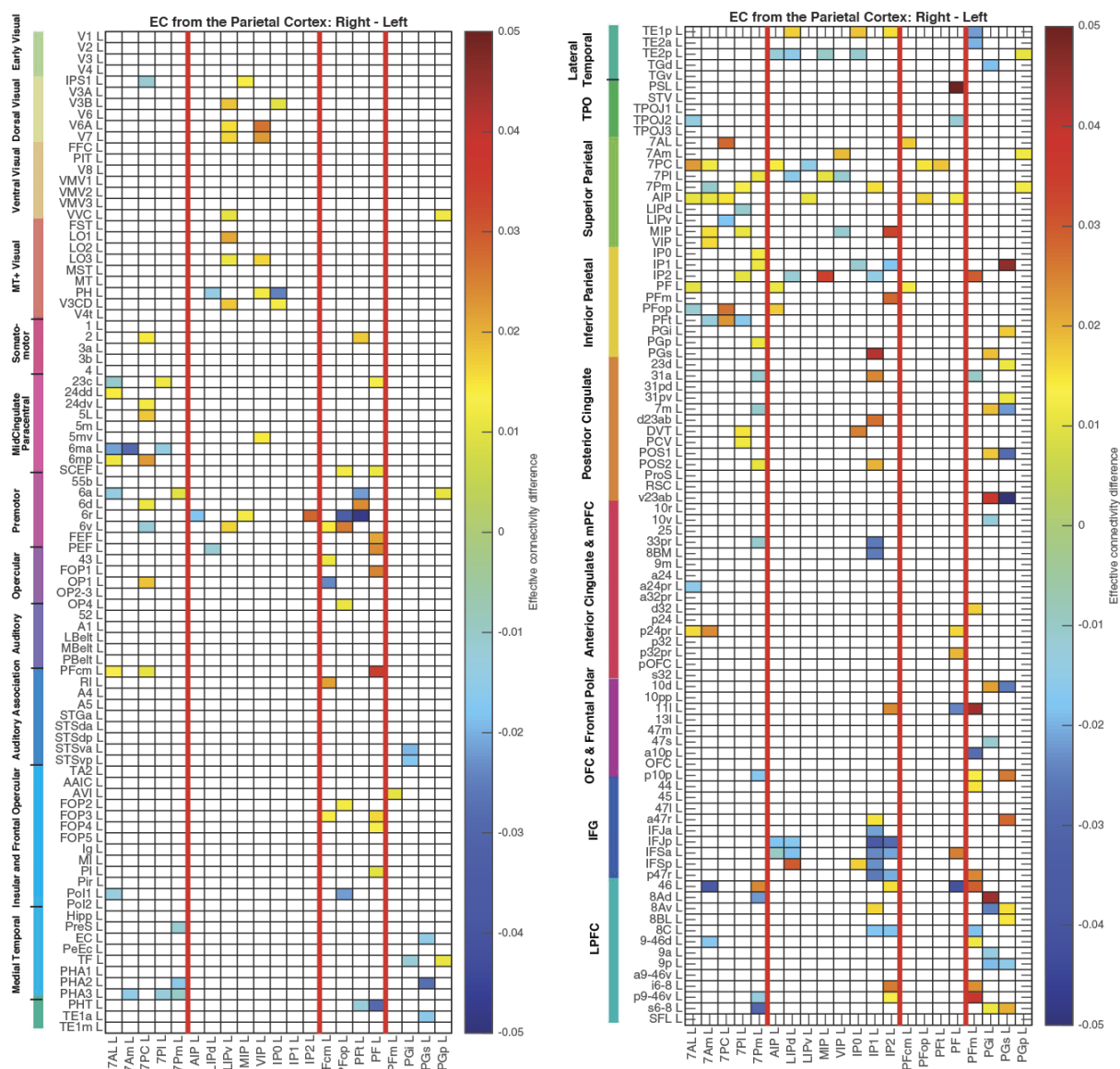
Fig. S7. Effective connectivity difference right hemisphere – left hemisphere FROM the posterior parietal cortex TO 180 cortical areas in the left hemisphere. The effective connectivity difference is read from column to row. Effective connectivity differences in the range -0.01 to 0.01 are shown as blank. Abbreviations: see Table S1. The four groups of posterior parietal cortex regions are separated by red lines.
