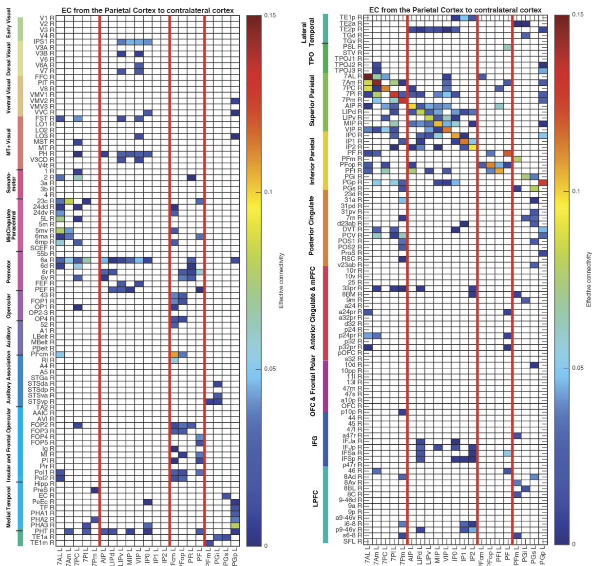
Fig. S3. Effective connectivity (EC) from the Left posterior parietal cortex to all 180 cortical areas in the Right hemisphere. All effective connectivities greater than 0 are shown, and effective connectivities of 0 are shown as a blank. The connectivities to the first set of cortical regions are shown on the left, and to the second set on the right. The four groups of posterior parietal cortex regions are separated by red lines. Abbreviations: see Table S1. The effective connectivity is read from column to row.
