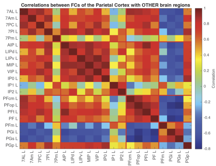
Fig. S5. Correlations between the functional connectivities with other cortical areas for the 21 different regions in the posterior parietal cortex. Abbreviations: see Table S1.
