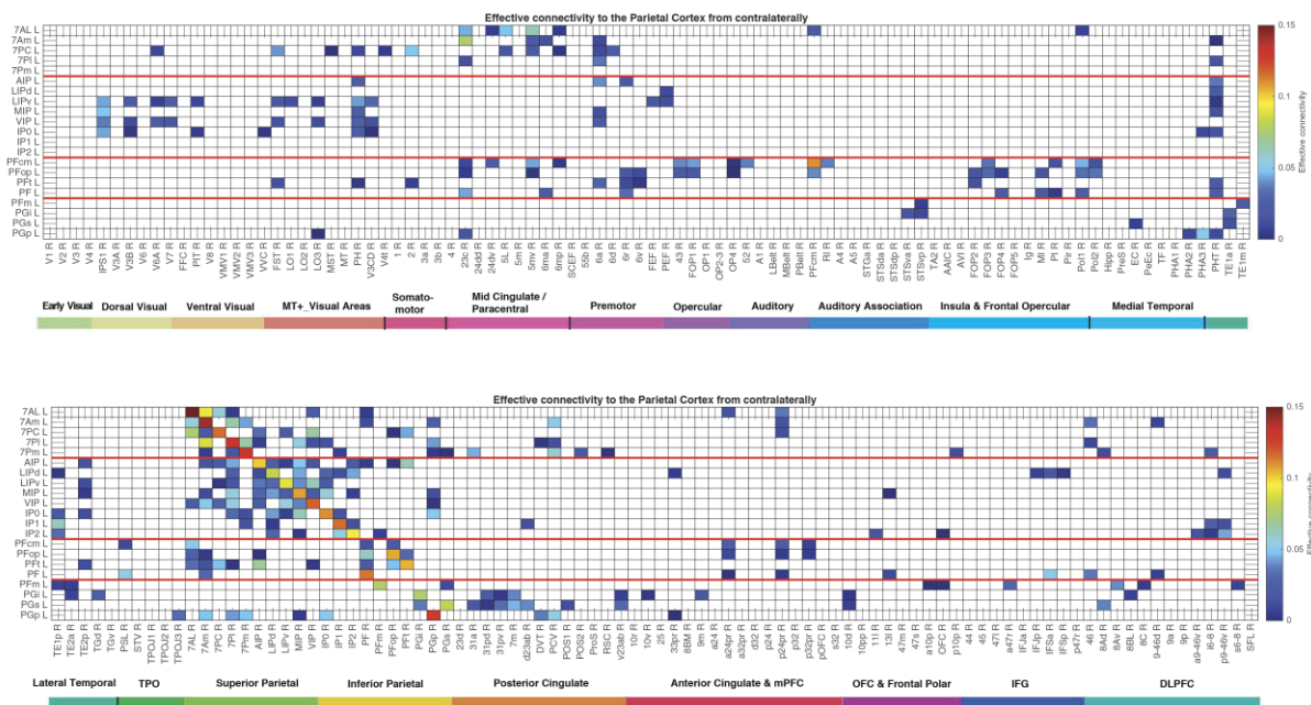
Fig. S2. Effective connectivity to the Left posterior parietal cortex from all 180 cortical areas in the Right hemisphere. All effective connectivities greater than 0 are shown, and effective connectivities of 0 are shown as a blank. The connectivities from the first set of cortical regions are shown above, and from the second set below, etc. The four groups of posterior parietal cortex areas are separated by red lines. Group 1 the superior parietal cortex is above the top red line. Group 2 the intraparietal cortex is below the top red line. Group 3 the somatosensory inferior parietal cortex areas is next. Group 4 the visual inferior parietal cortex regions is below the lowest red line. Abbreviations: see Table S1. The effective connectivity is read from column to row.
